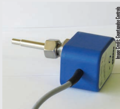
The compact plug and play EGE SNS 450 thermodynamic flow sensor provides ease of flow monitoring with low maintenance benefits.
